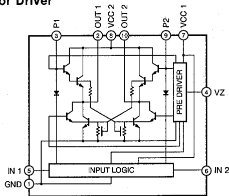
IC301, 302 : LB1641 Motor Driver
