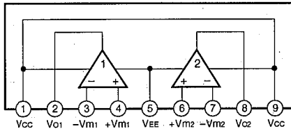
IC802 : \mu PC4570HA Dual OP-Amp
