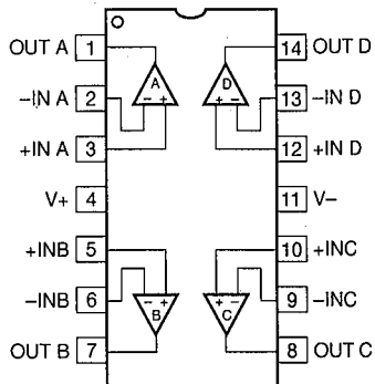
IC13, 14, 24, 25, 501, 502 : \mu PC4574G2 (FUNCTION) IC31 : \mu PC4574G2 (DSP) 4-Channel OP-Amp
