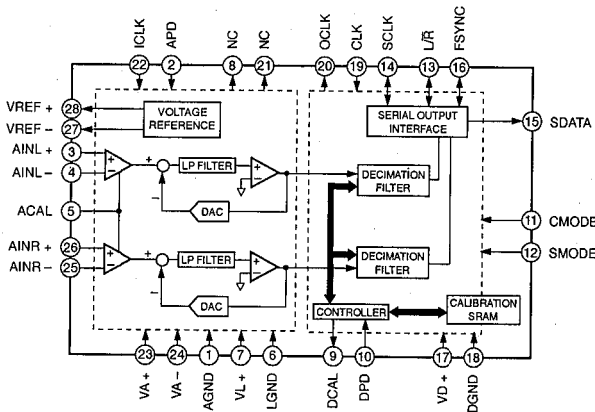
IC24 : AK5390-VS 20 bit 2-Channel A/D Converter
