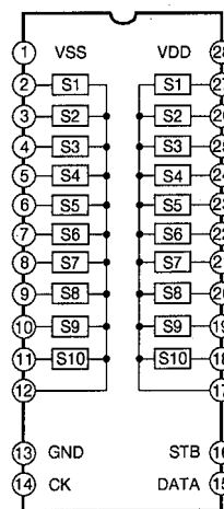
IC403, 405 : TC9273N-004 Analog Function Switch
