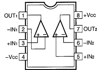
IC1 : MC14577CP (DSP) IC3, 37~40 : \mu PC4570G2 (DSP) IC4, 5 : NJM2904G (DSP) IC3, 4, 9~12, 15, 21~23 : \mu PC4570G2 (FUNCTION) IC5~8 : NJM2068MD (FUNCTION) Dual OP-Amp
