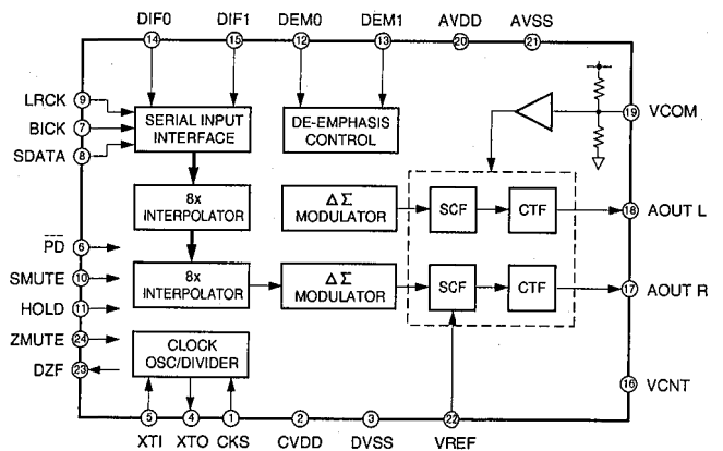
IC25~28 : AK4320-VM 1 bit D/A Converter
